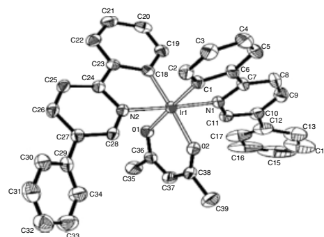
Figure 2. ORTEP diagram of (dppy) 2 Ir(acac).
